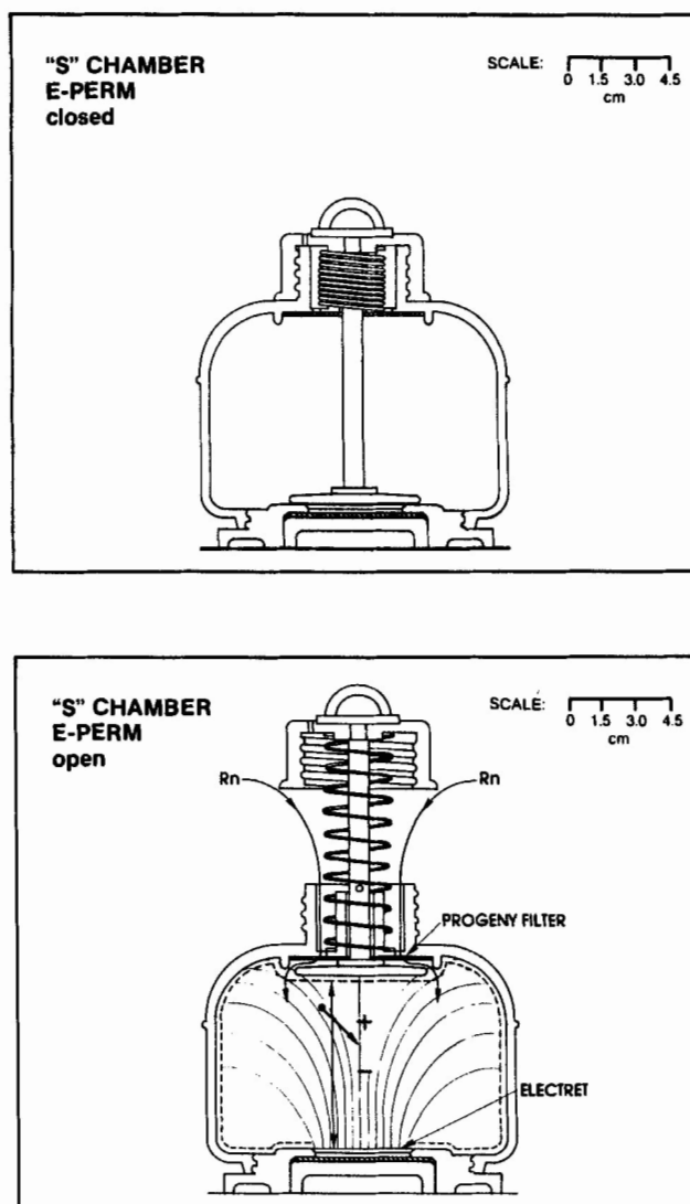
Fig. 1. Schematic of electret ion chamber-based E-PERM ^{222}\text{Rn} gas monitor. Upper window shows the E-PERM in its "off" position and the lower window shows the E-PERM in its "on" position.
